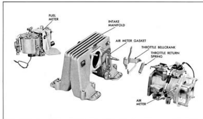
Fig. 12 Fuel Injection Basic Components
